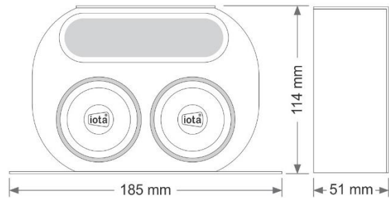
All dimension are in mm tolerance ±0.2mm
